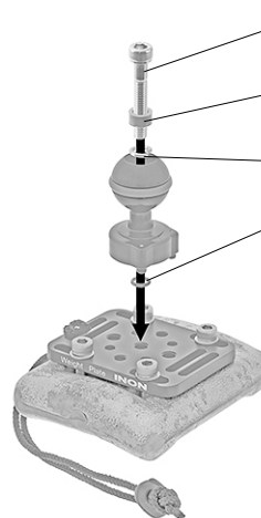
M6 Cap Screw [preinstalled on Direct Base Ⅲ]
