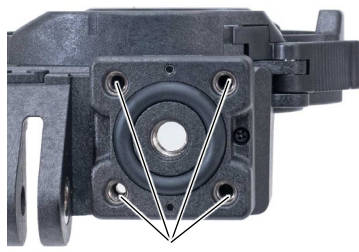
Male Adapter fixing holes
